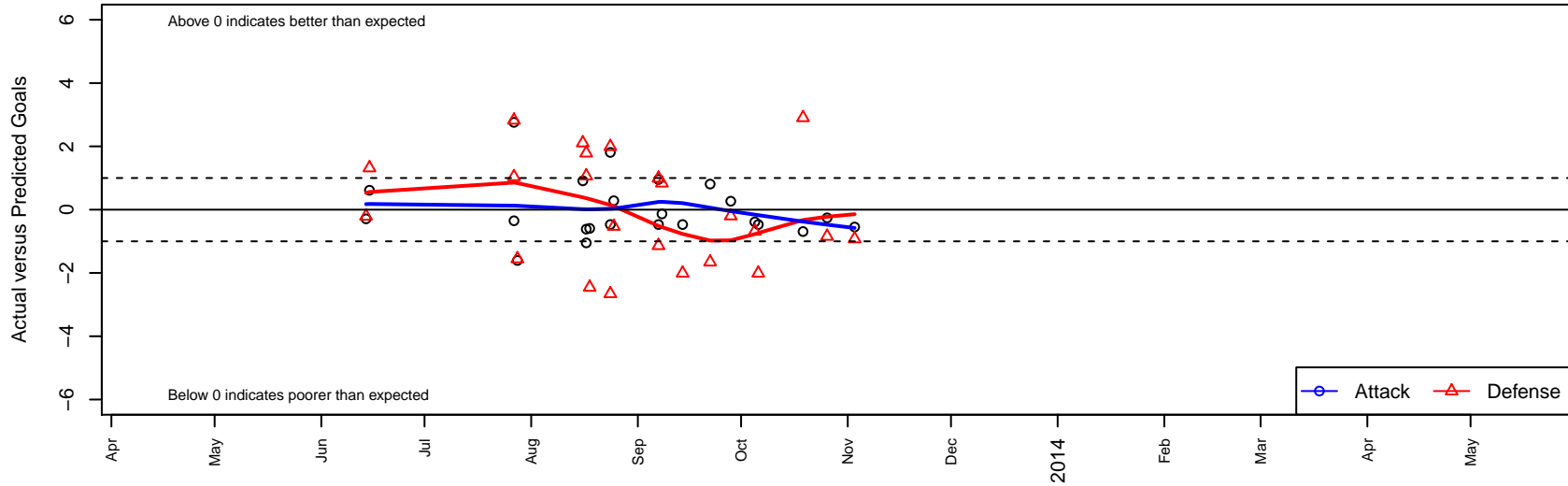
FC Spokane White B00 Dots are actual minus expected GF (blue circles) and GA (red triangles). Blue line is smoothed change in attack strength. Red is smoothed change in defense strength.
